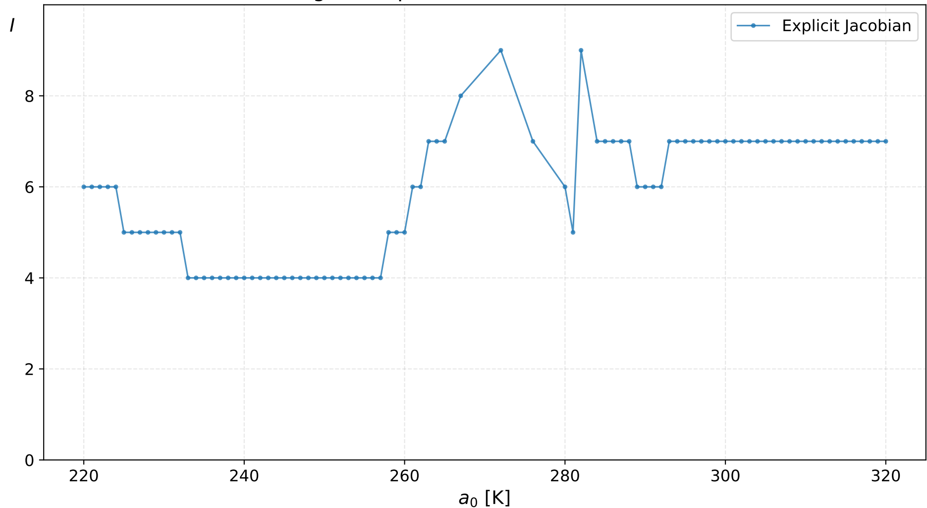
Convergence Speed: Iterations vs Initial Guess
